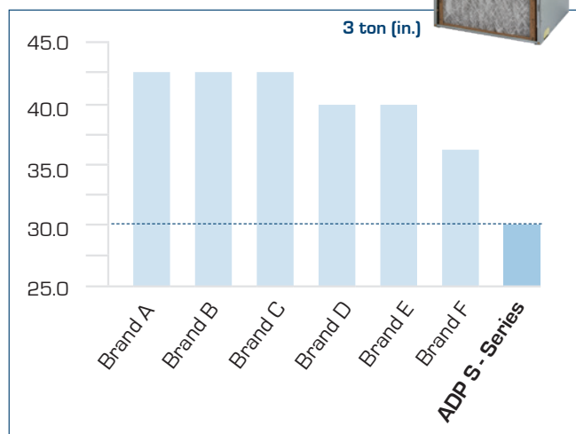
Wall Mount Air Handler Height Comparison
