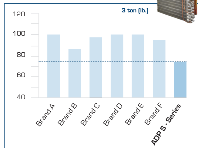
Aluminum Wall Mount Air Handler Weight Comparison
