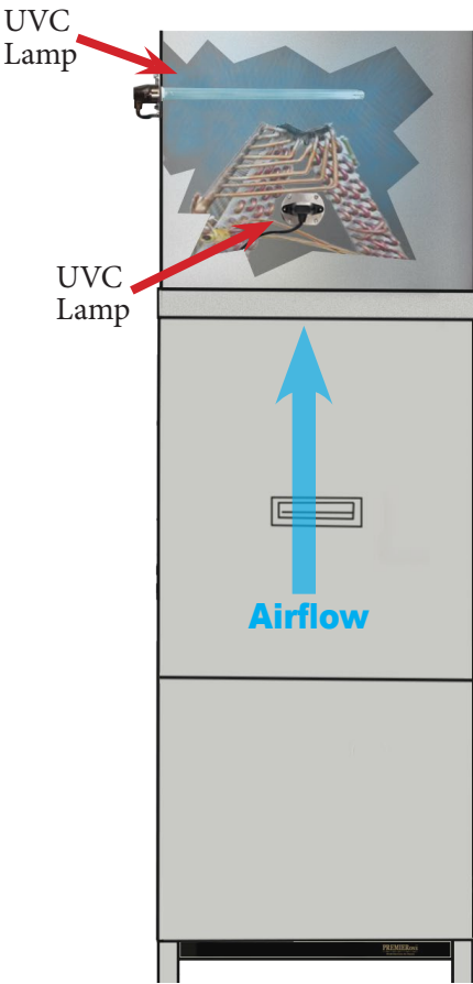
MUV7-100DR shown mounted on a heat pump.
